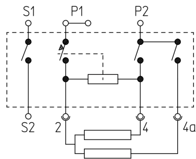
Internal circuit diagram in "OFF"-position
